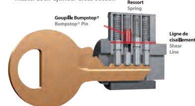
Coupe transversale du cylindre Master Lock® Master Lock® Cylinder Cross-section
